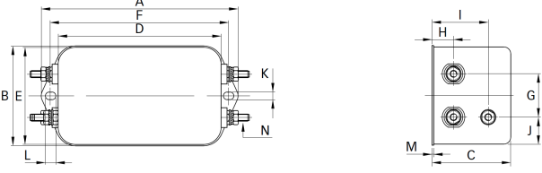
Connection style -08, 16 to 30 A types
